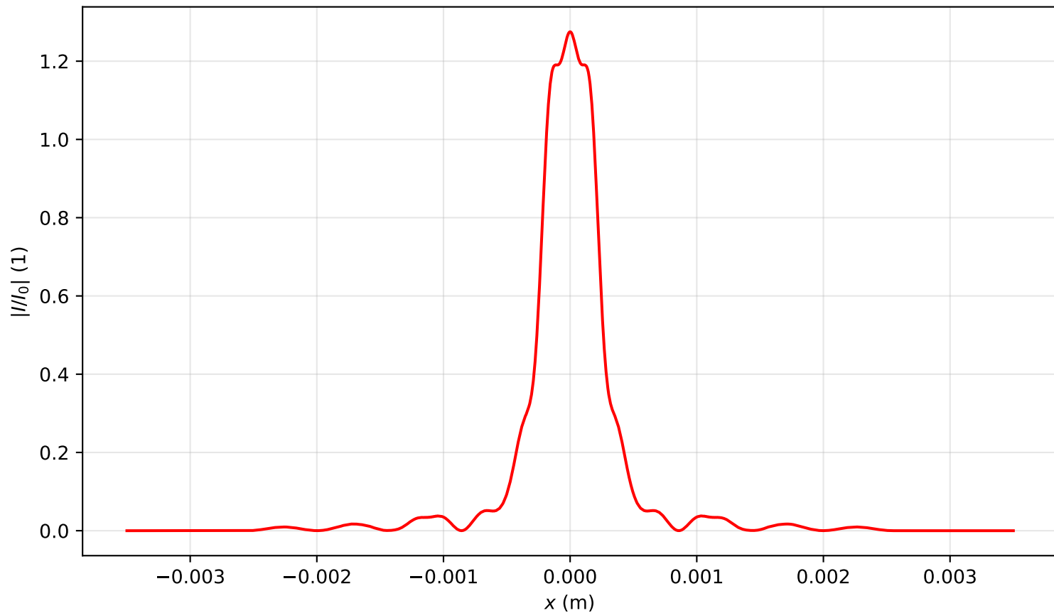
Intensity profile I(x, y = 0, z = 0.478)/I_0 , P_{in}=3.0P_{cr} , artificial time
